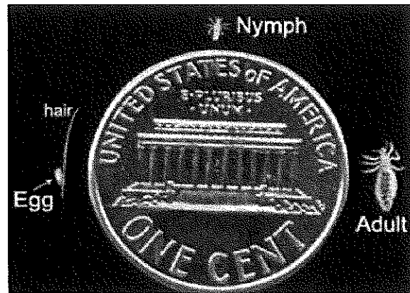
Actual size of the three lice forms compared to a penny (CDC Photo)
